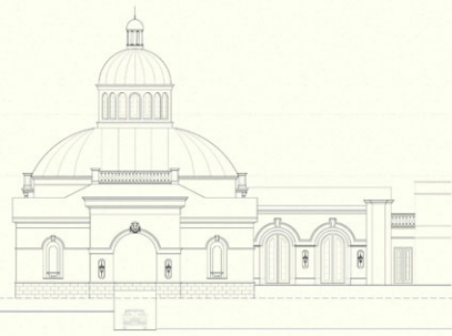
WEST ELEVATION
